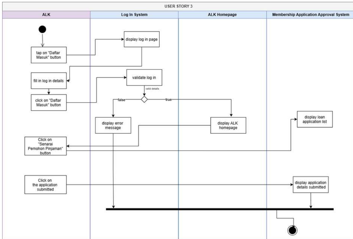
Figure 44: Activity diagram for ALK view validated loan application
