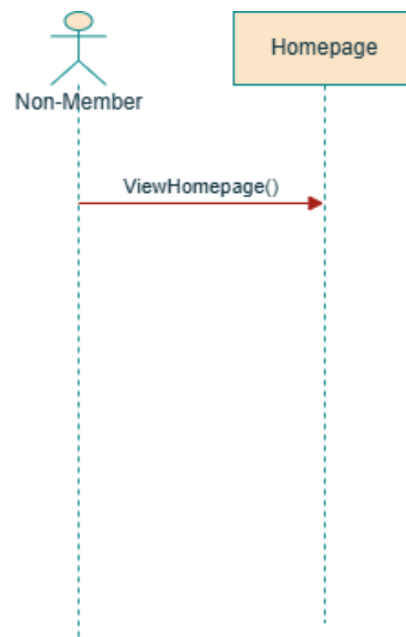
Figure 138: TC004_02: Test <View Homepage (SD027)>
