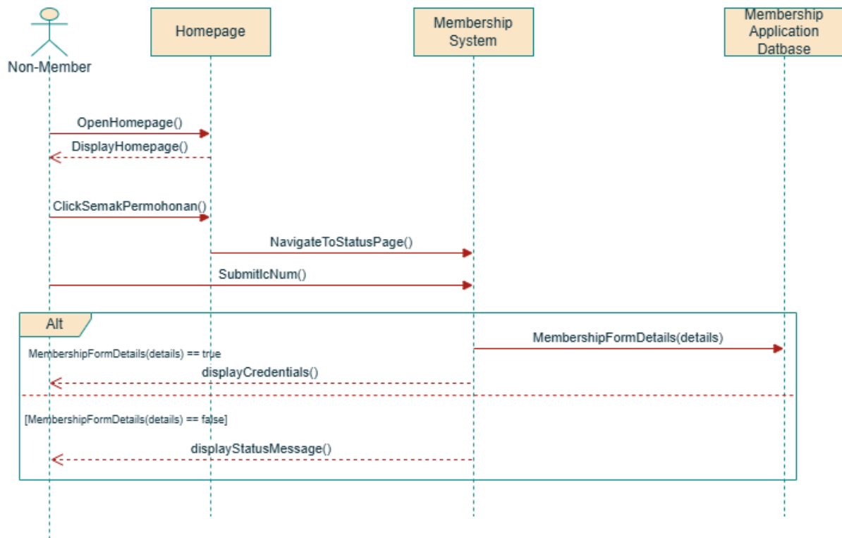
Figure 139: TC004_03: Test <Get Member Approval (SD028)>
