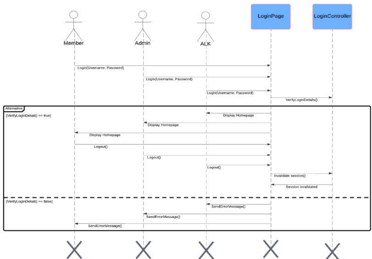
Figure 68: SD024 sequence diagram for Authentication module
