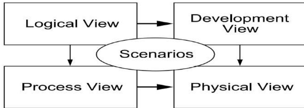
Figure 52: Architectural Views
