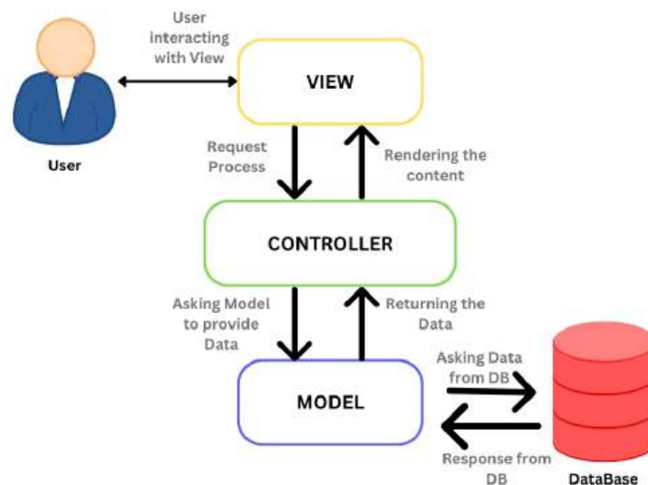
Figure 51: MVC organization
