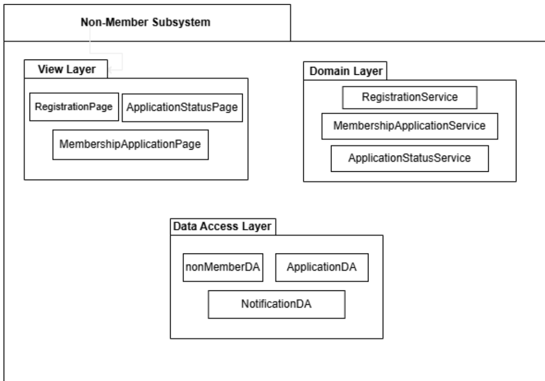
Figure 57: Package diagram for Non-Member subsystem
