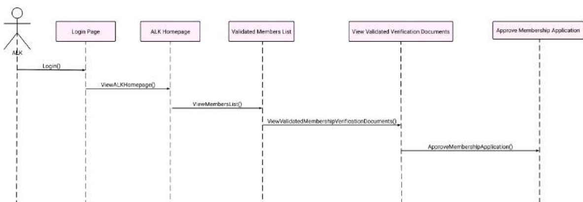
Figure 133: TC003_04: Test <Approve Member Application (SD019)>
