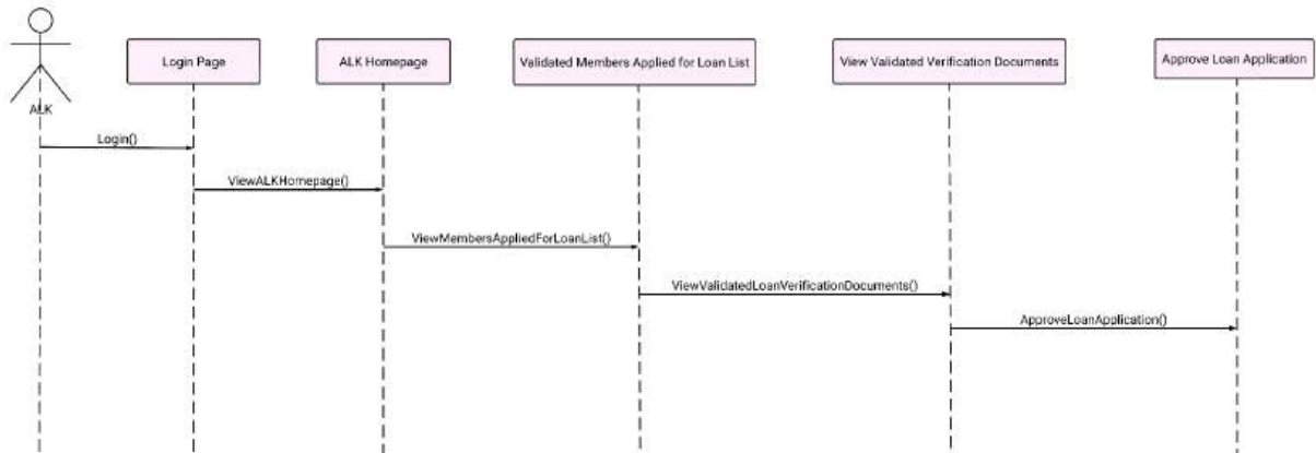
Figure 134: TC003_05: Test <Approve Loan Application (SD020)>
