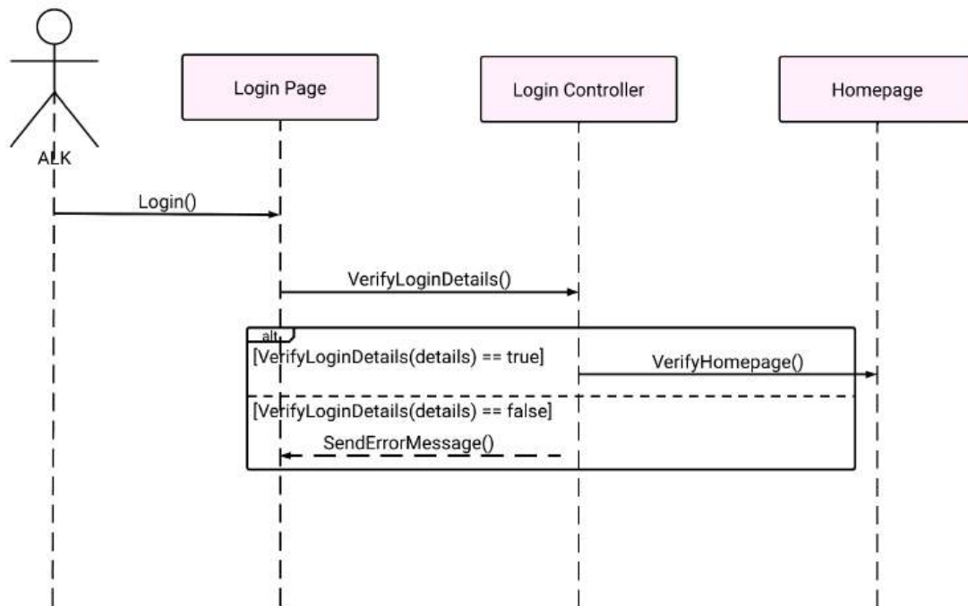
Figure 140: TC005_01: Test <Log in (SD029)>
