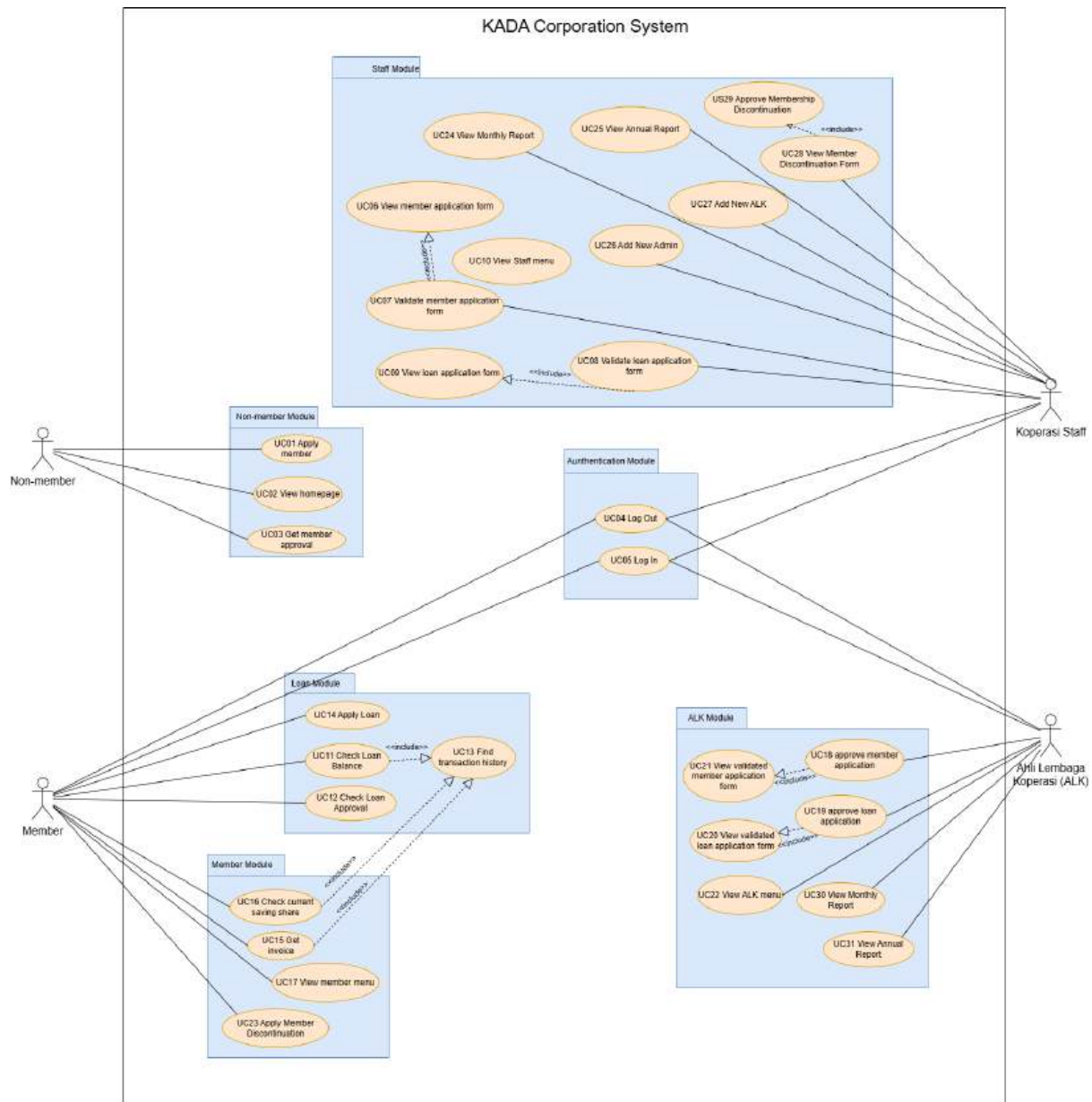
Figure 53: Use case diagram for Koperasi KADA System
