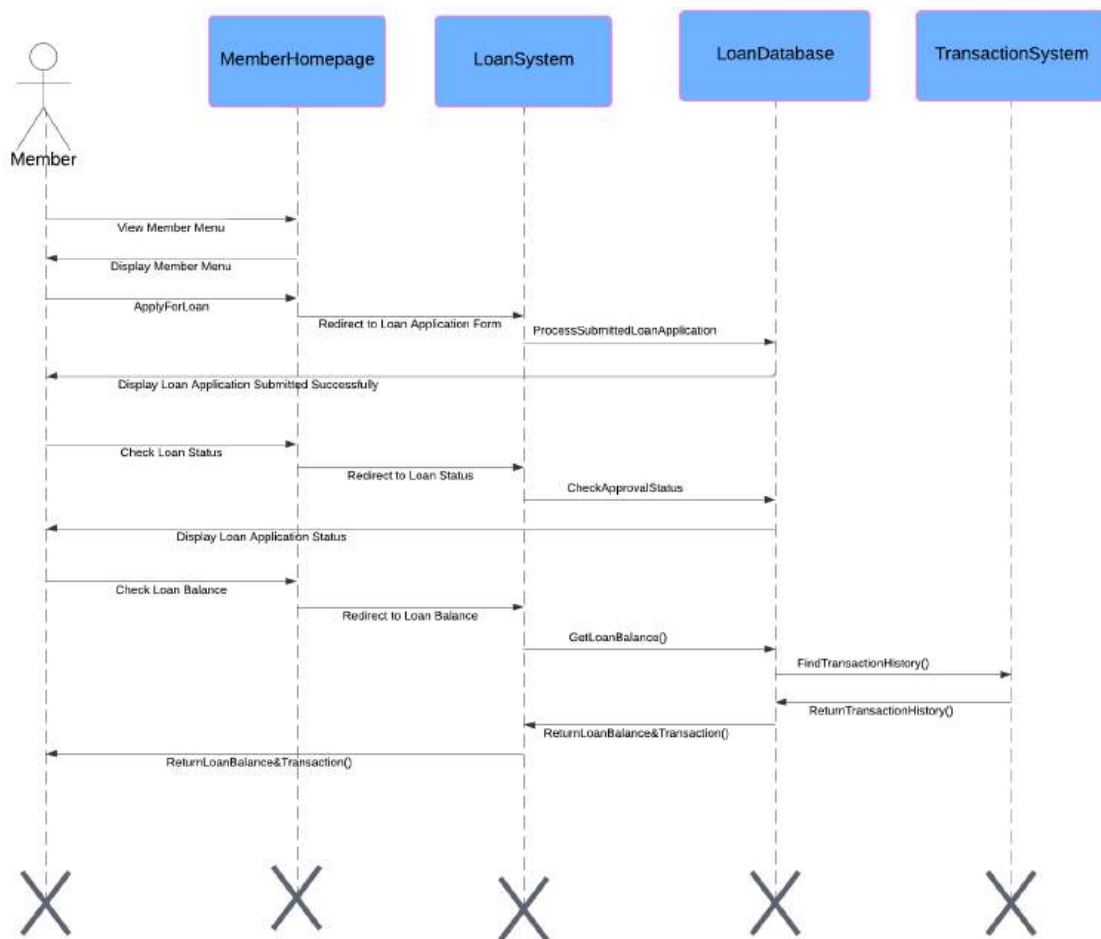
Figure 71: SD027 sequence diagram for Loan module
