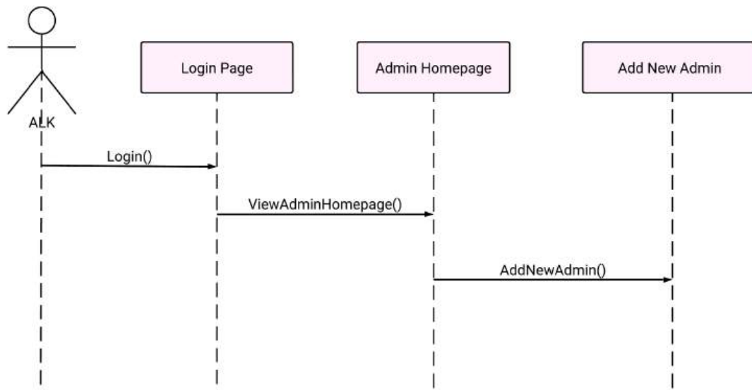
Figure 25: SD015 sequence diagram for add new admin
