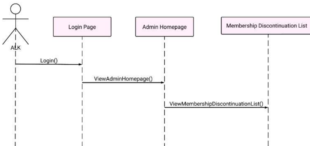
Figure 19: SD009 sequence diagram for view membership termination application form
