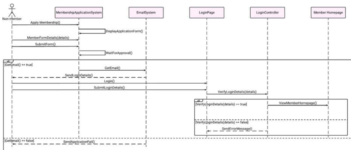
Figure 49: SD023 Sequence diagram for non-member apply for membership
