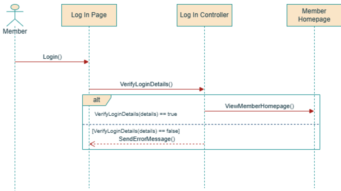
Figure 116: TC001_01: Test <View Member Menu (SD024)>
