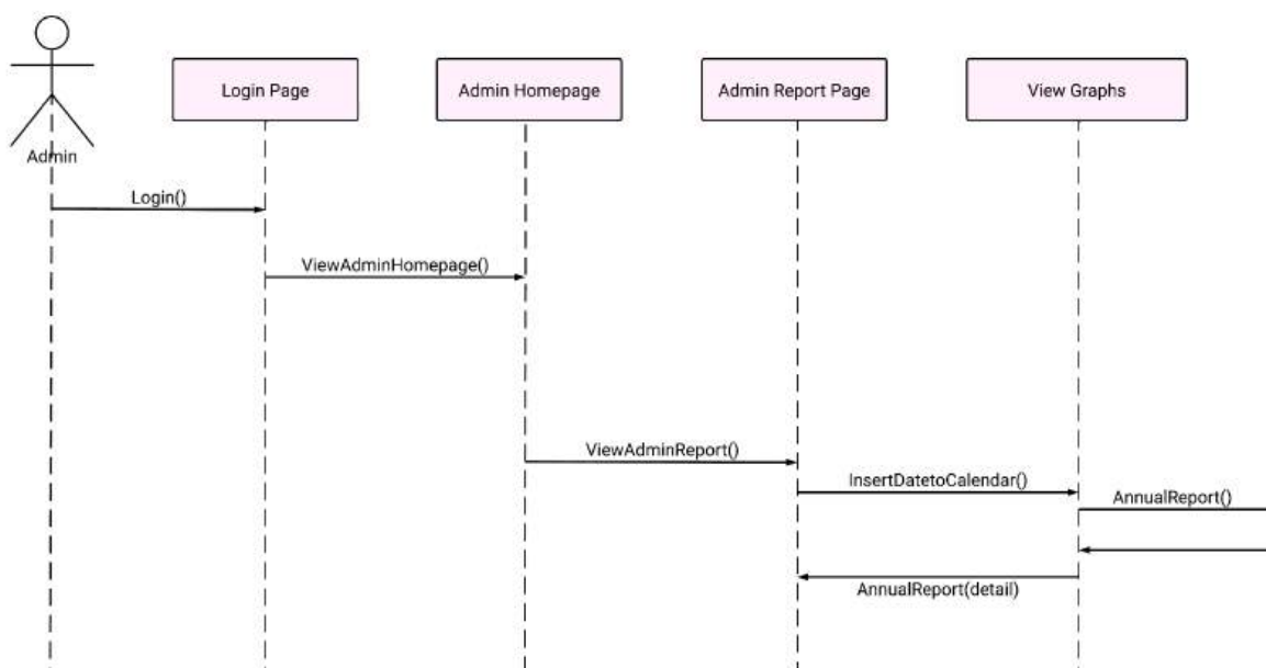
Figure 127: TC002_09: Test <View Annual Report (SD014)>
