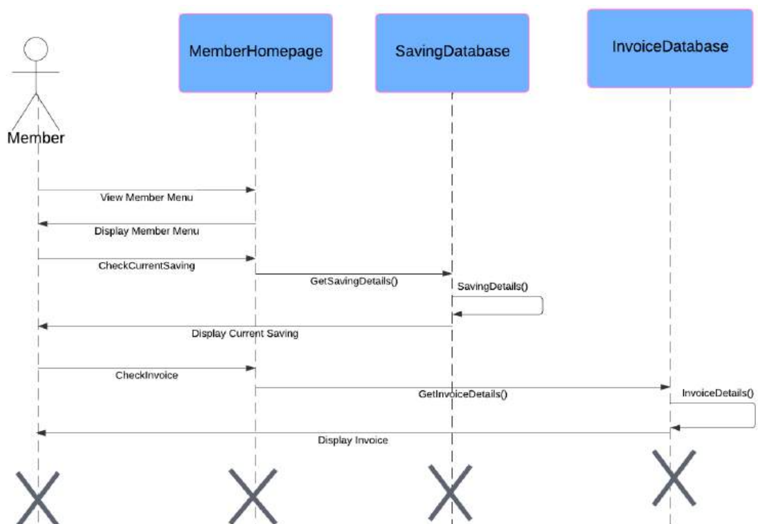
Figure 70: SD026 sequence diagram for Member module
