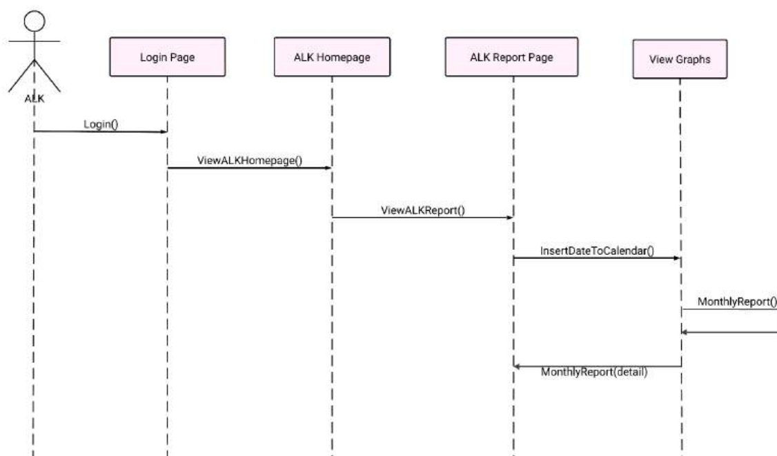
Figure 135: TC003_06: Test <View Monthly Report (SD021)>
