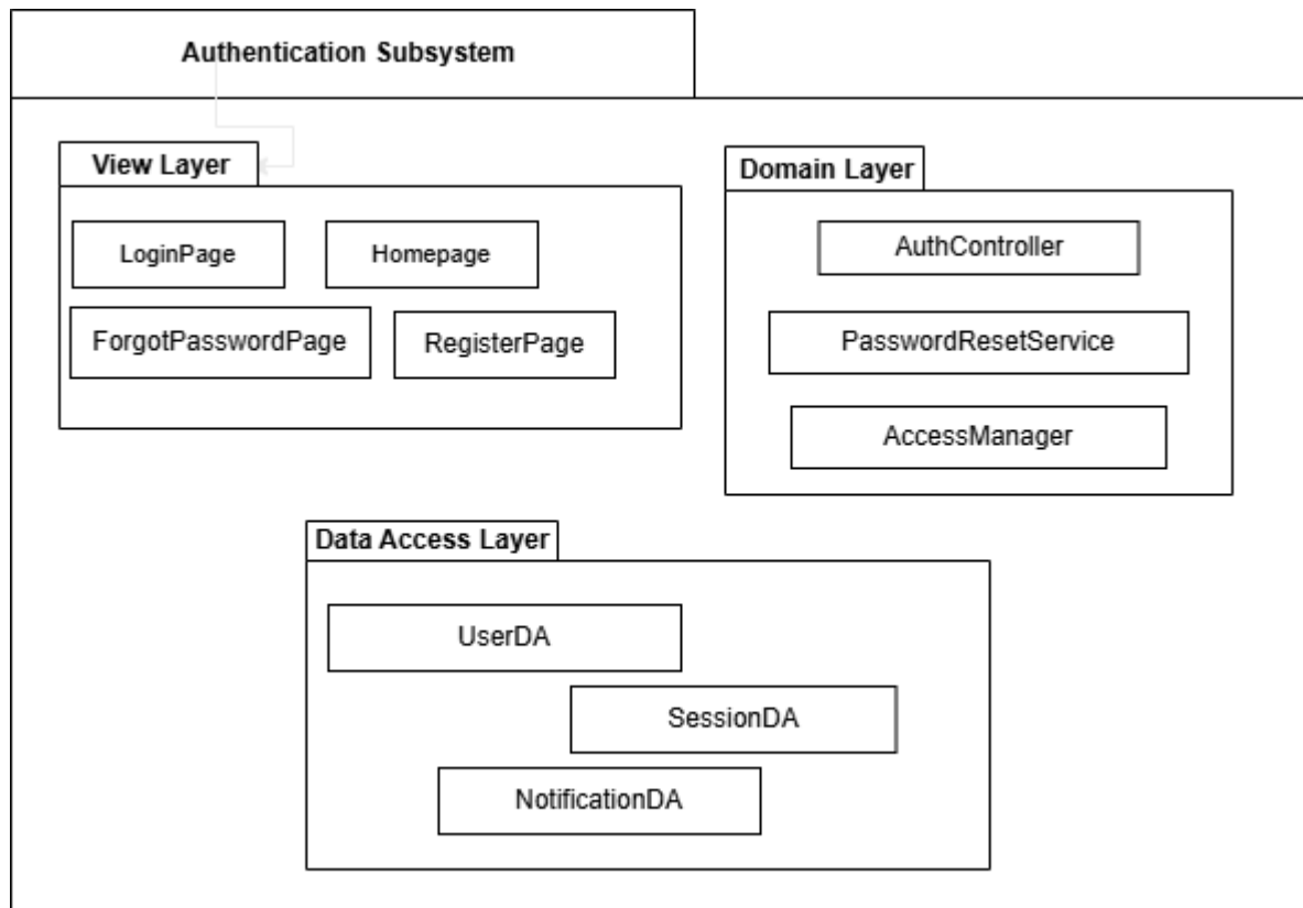
Figure 60: Package diagram for Authentication subsystem
