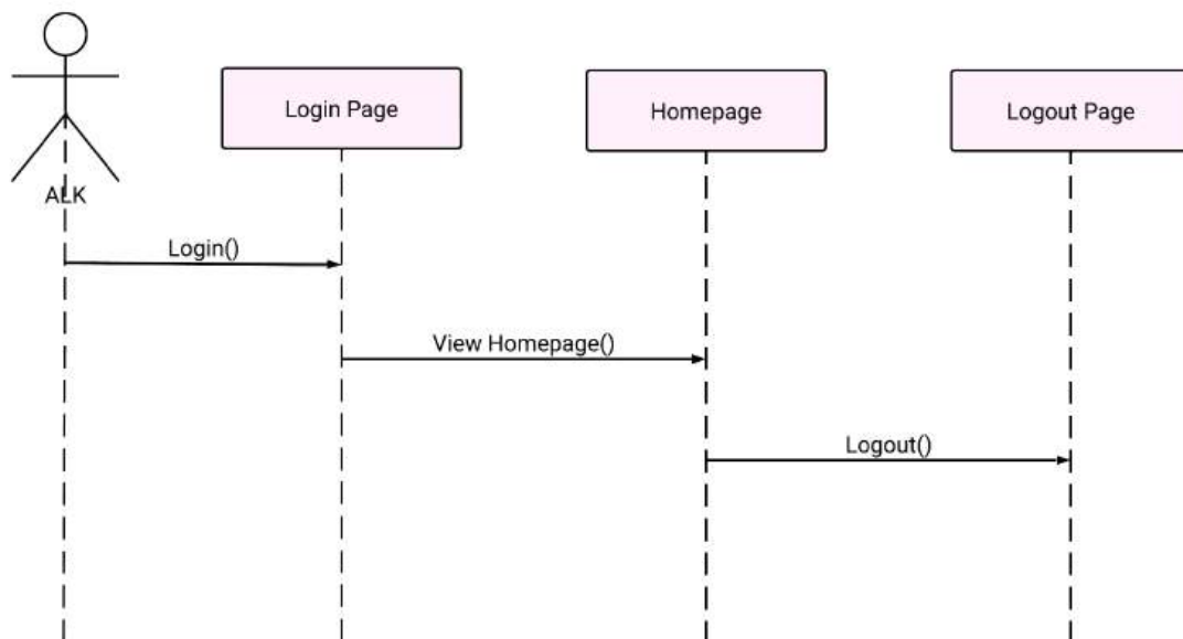
Figure 141: TC005_02: Test <Log out (SD030)>
