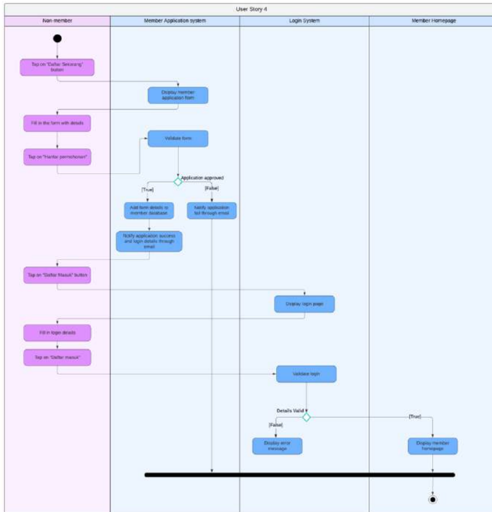
Figure 50: Activity diagram for non-member apply membership
