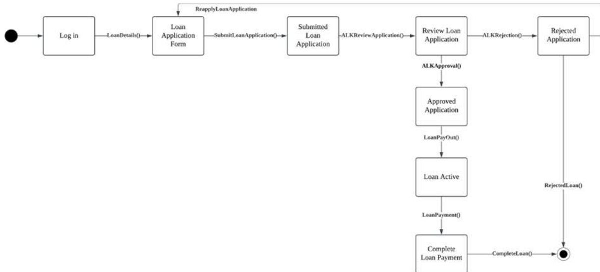
Figure 4: State Machine Diagram for <Loan Application System>
