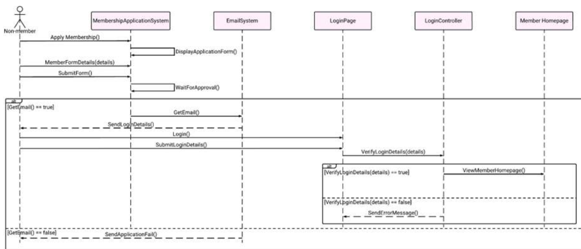
Figure 137: TC004_01: Test <Apply Membership (SD023)>
