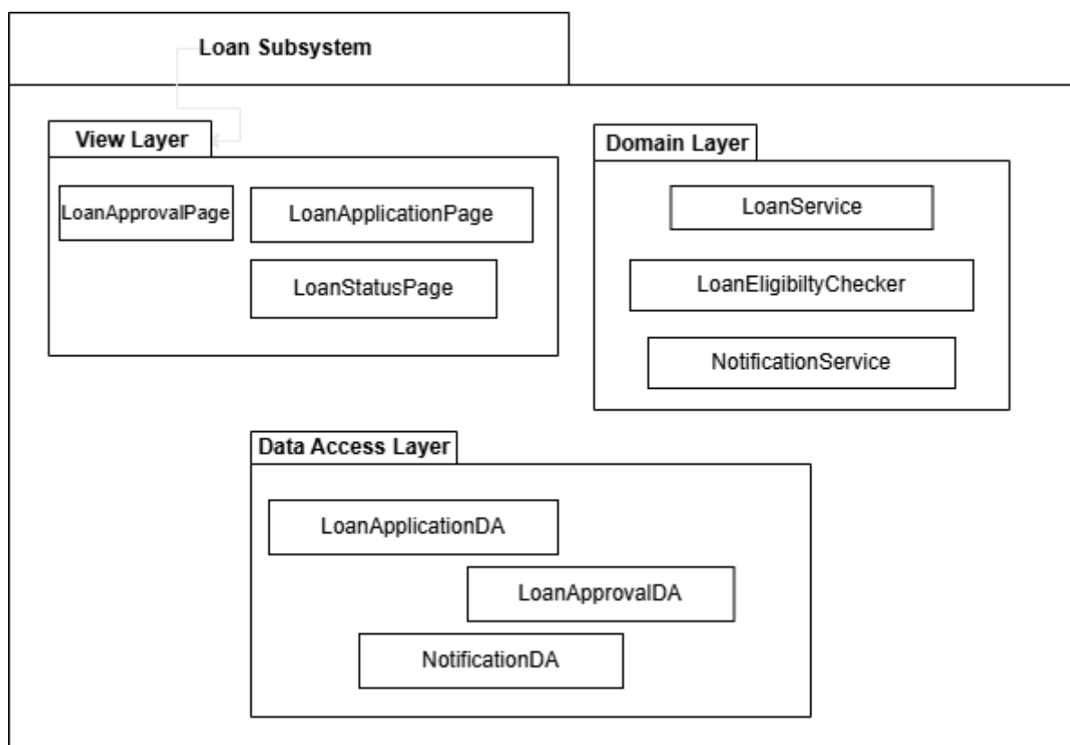
Figure 61: Package diagram for Loan subsystem
