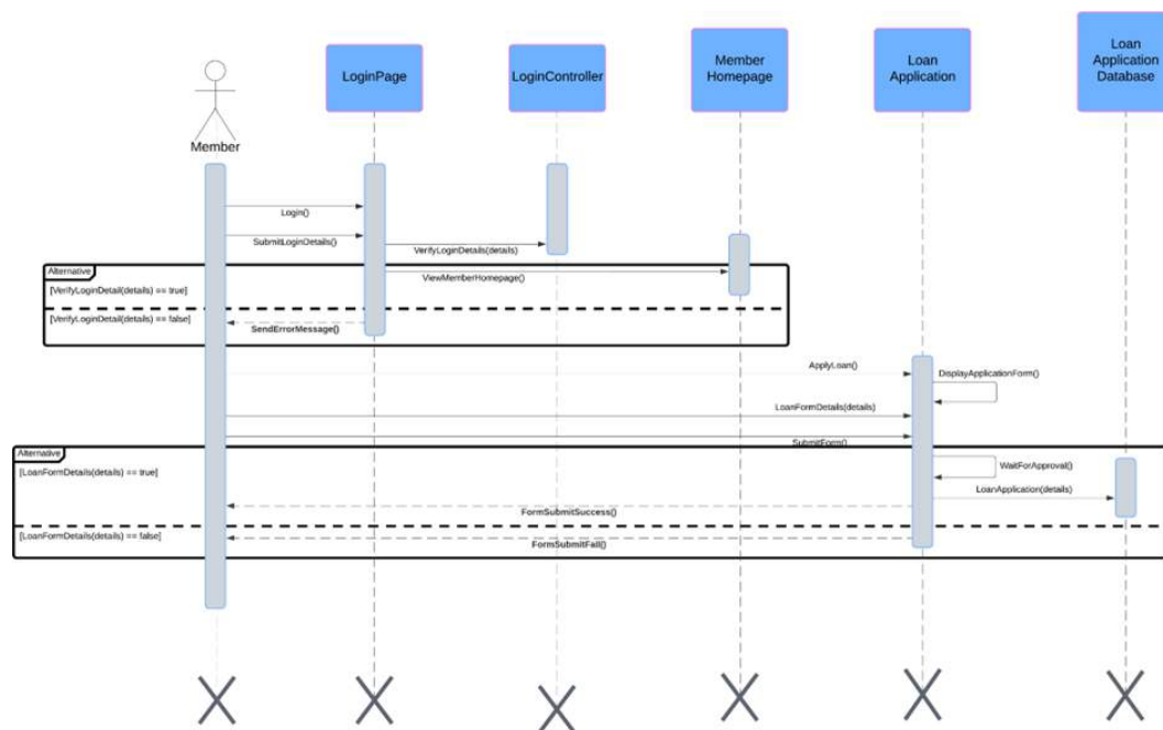
Figure 142: TC006_01: Test <Apply Loan (SD001)>
