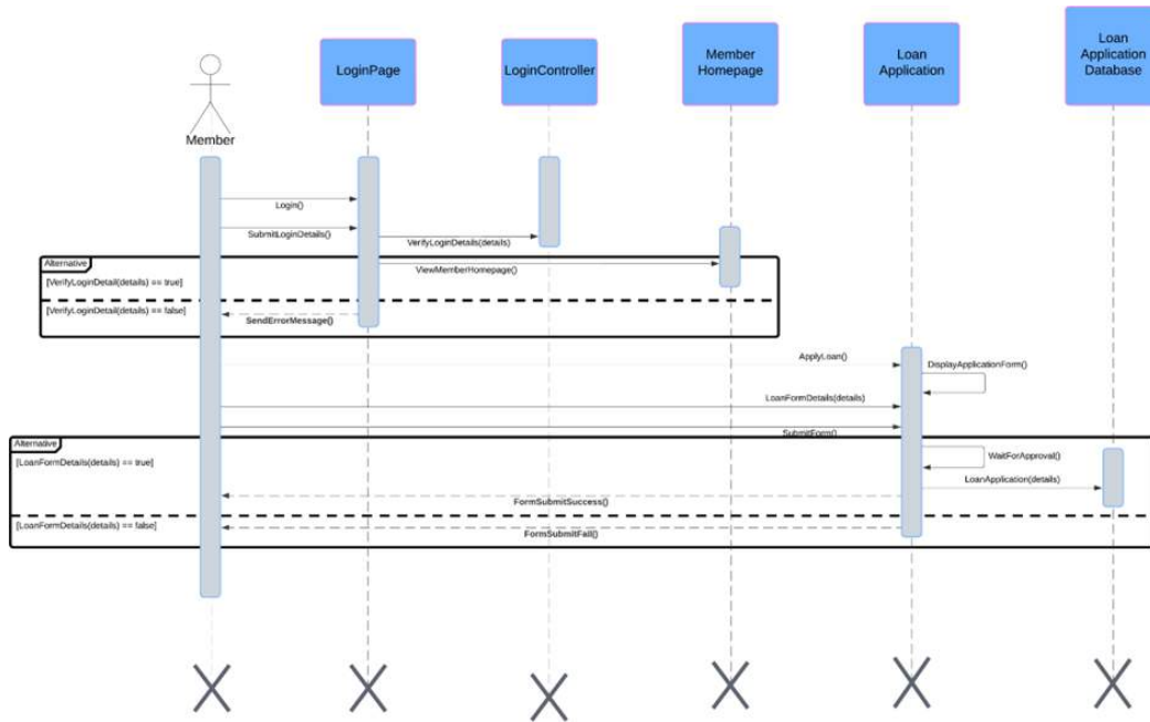
Figure 143: TC006_02: Test <Check Loan Approval (SD002)>
