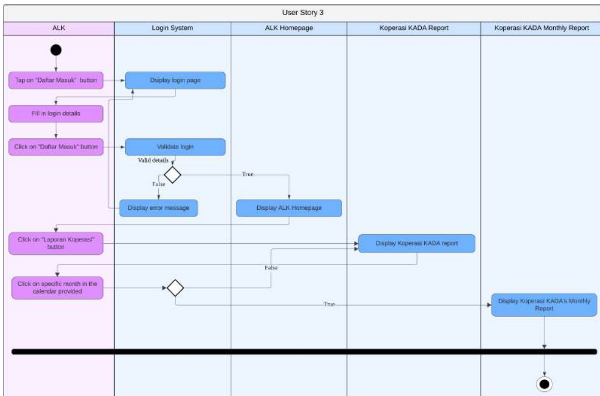
Figure 47: Activity diagram for ALK view monthly report
