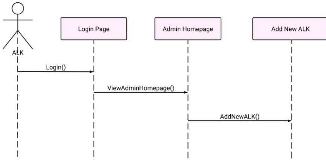
Figure 129: TC002_11: Test <Add New ALK (SD016)>
