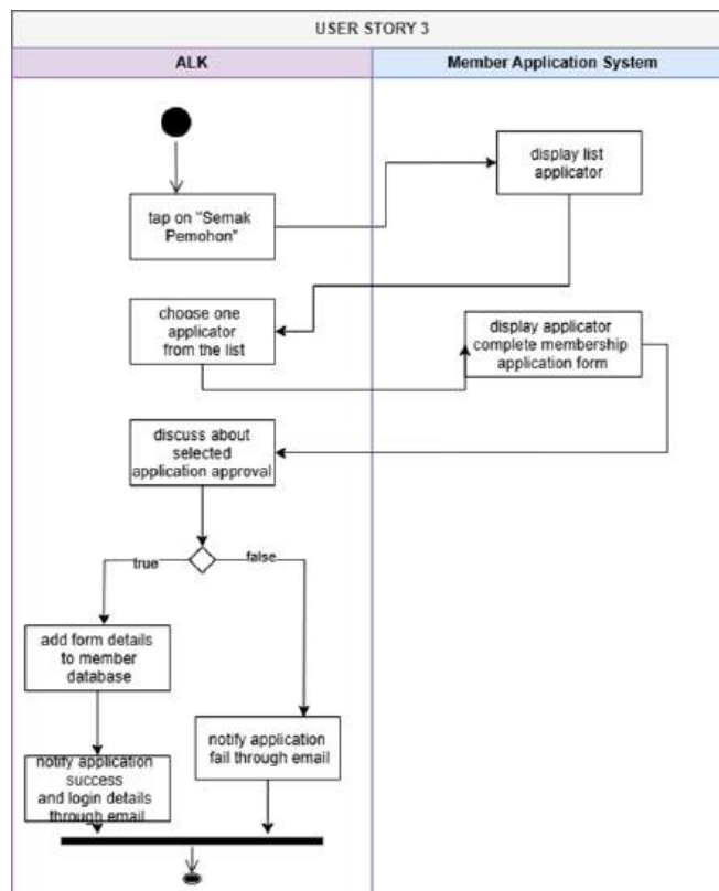
Figure 45: Activity diagram for ALK approve member application
