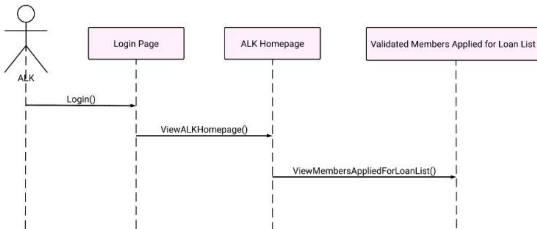
Figure 38: SD018 Sequence diagram for ALK view validated loan applications
