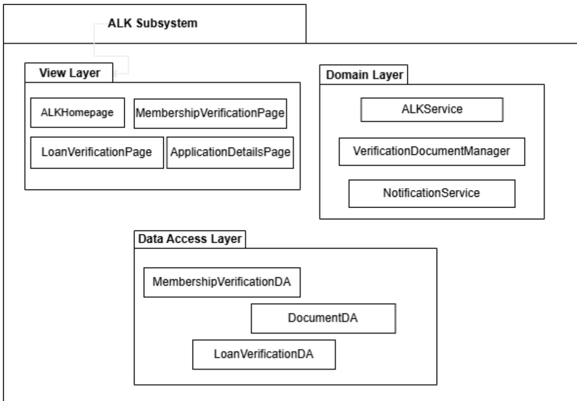
Figure 59: Package diagram for ALK subsystem
