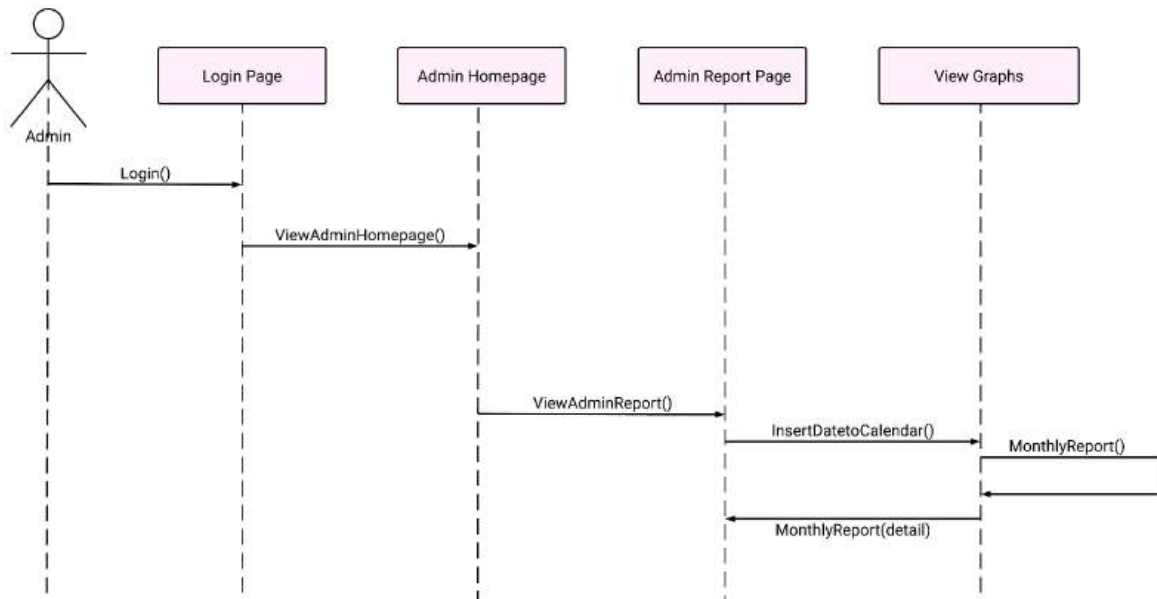
Figure 126: TC002_08: Test <View Monthly Report (SD013)>
