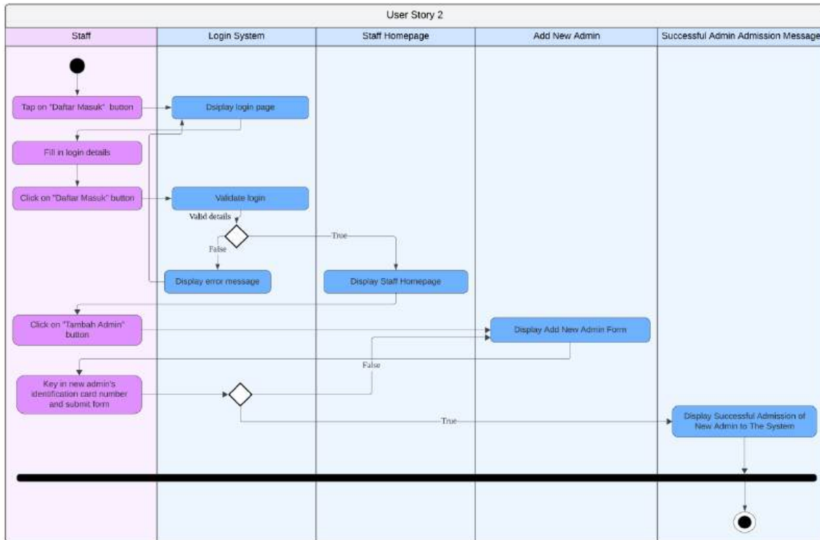
Figure 35: Activity diagram for when admin chooses to add new admin to the system
