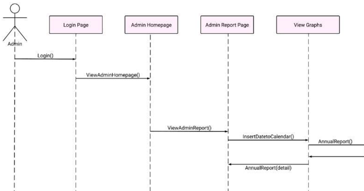
Figure 24: SD014 sequence diagram for view annual report
