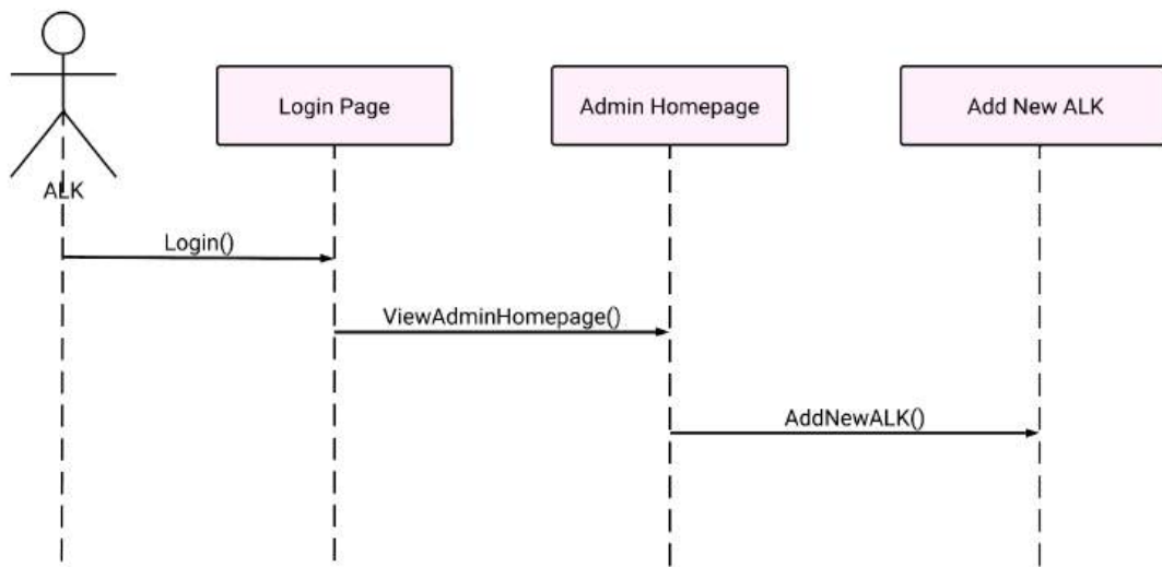
Figure 26: SD016 sequence diagram for add new ALK
