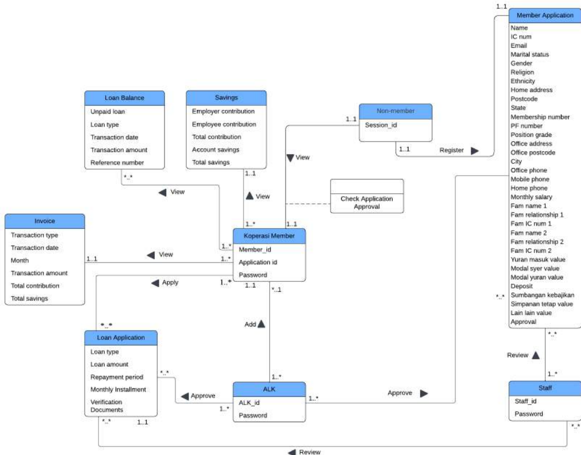
Figure 75: Global conceptual entity relationship diagram design
