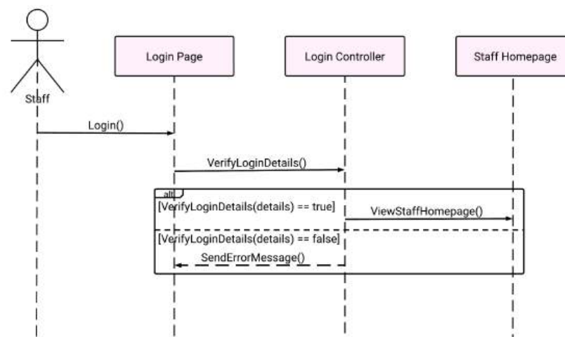
Figure 119: TC002_01: Test <View Staff Menu (SD025)>
