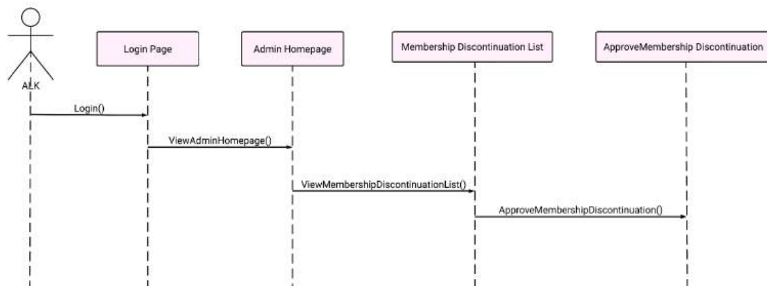
Figure 22: SD012 sequence diagram for approve membership termination application form
