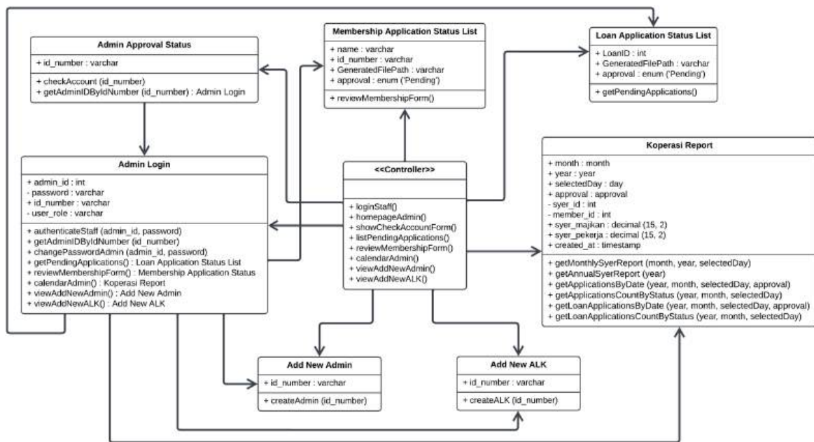
Figure 64: Class diagram for Admin module
