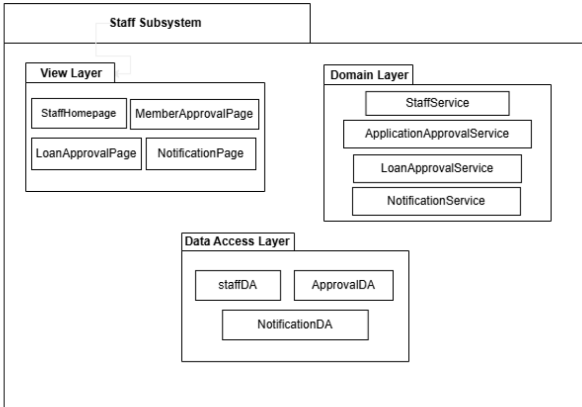
Figure 58: Package diagram for Staff subsystem
