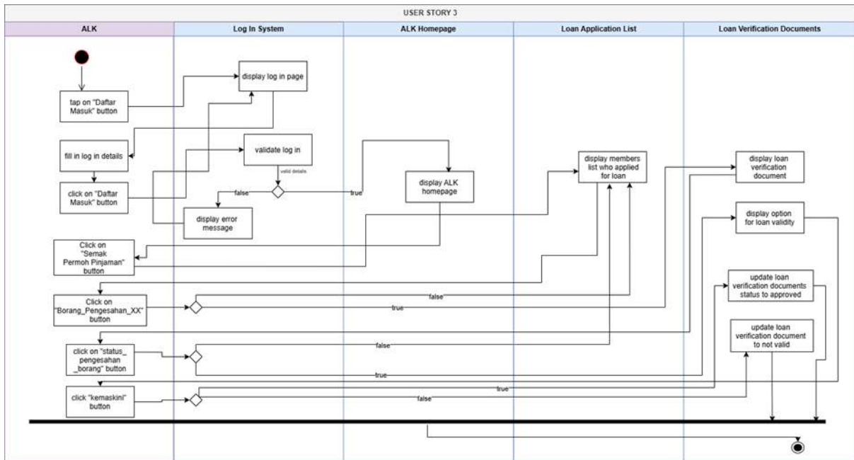
Figure 46: Activity diagram for ALK approve loan application
