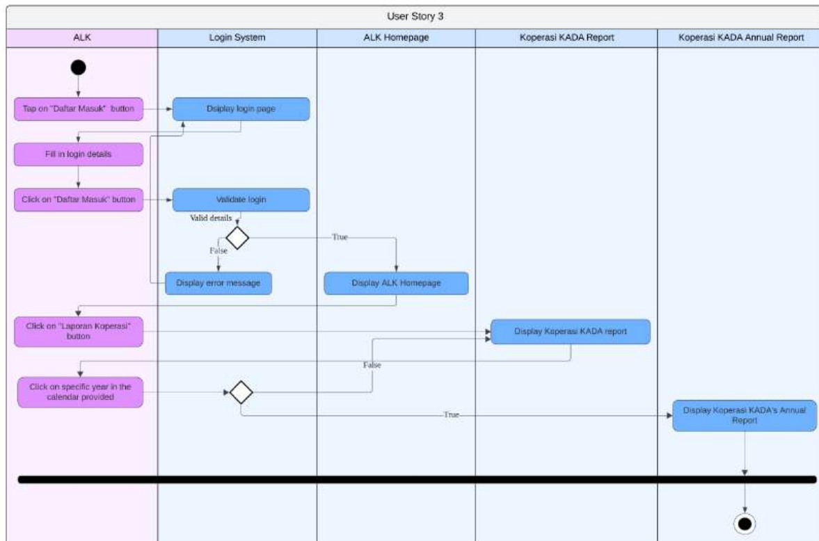
Figure 48: Activity diagram for ALK view annual report
