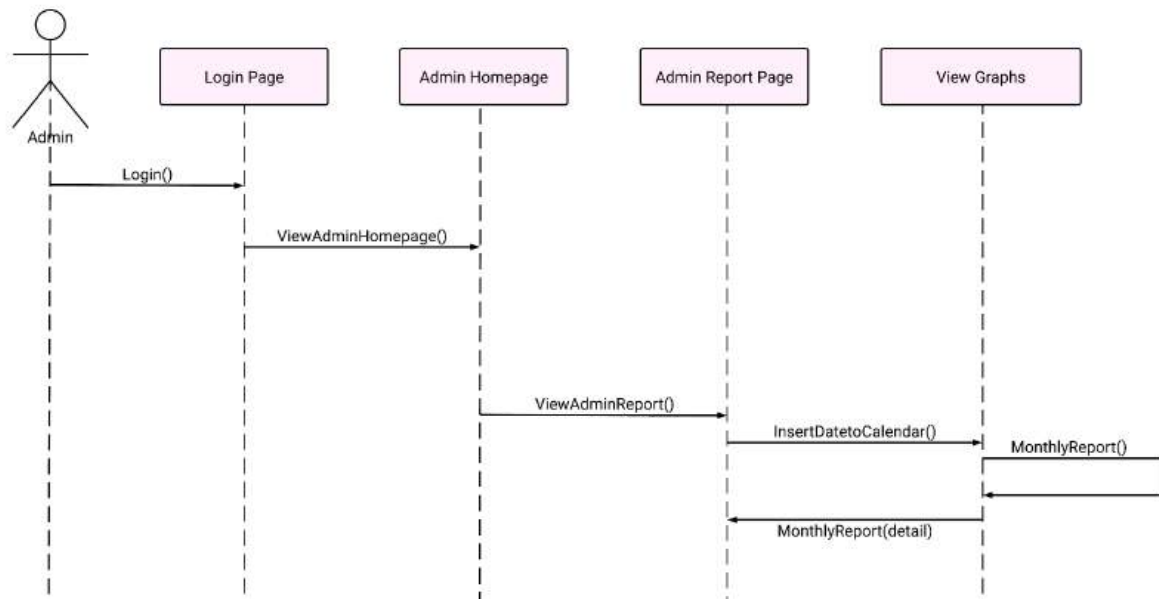
Figure 23: SD013 sequence diagram for view monthly report
