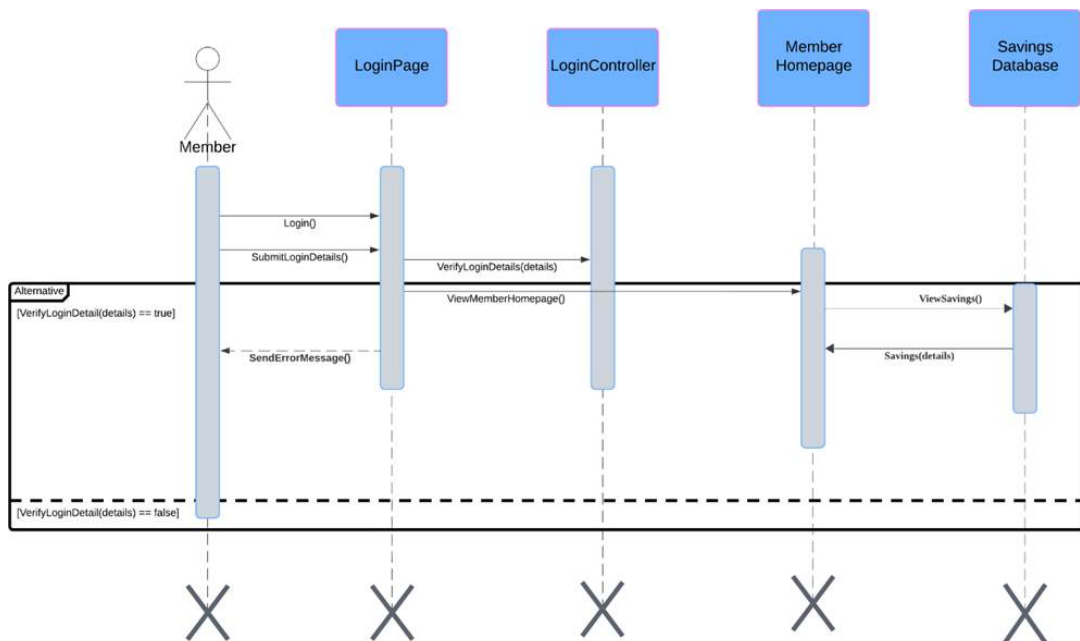
Figure 117: TC001_02: Test <Check Current Saving (SD003)>
