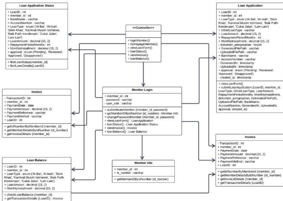
Figure 67: Class diagram for Loan module
