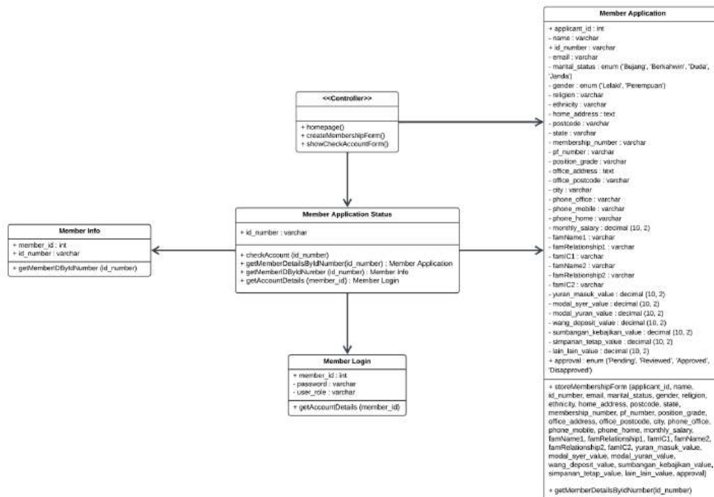
Figure 63: Class diagram for Non-Member module
