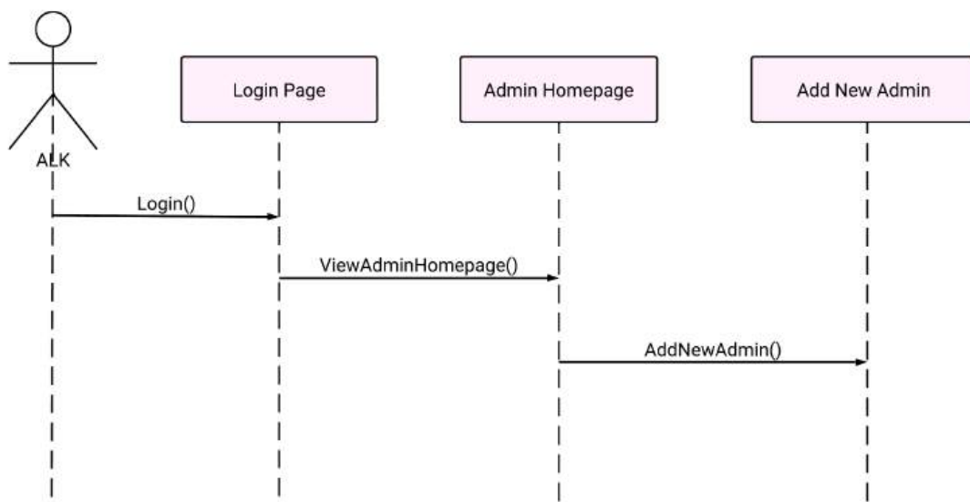
Figure 128: TC002_10: Test <Add New Admin (SD015)>
