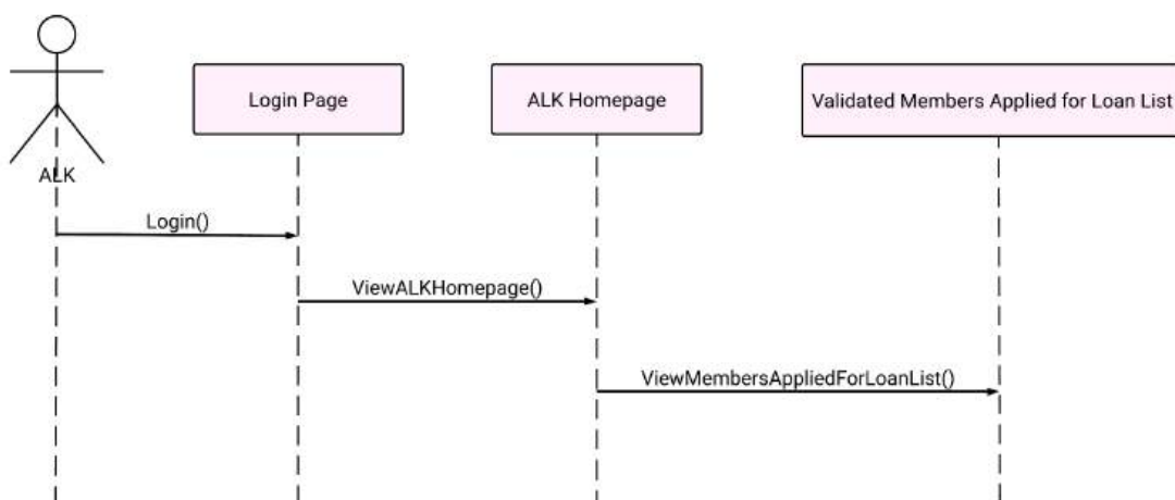
Figure 132: TC003_03: Test <View Validated Loan Application Form (SD018)>
