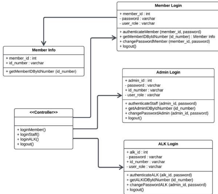
Figure 66: Class diagram for Authentication module
