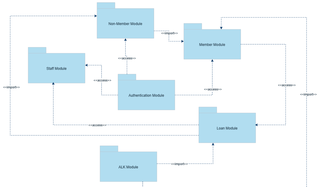
Figure 55: Package diagram for Koperasi KADA membership and loan application system
