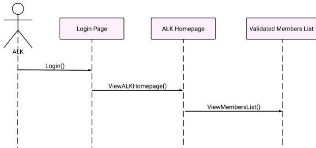
Figure 37: SD017 Sequence diagram for ALK view validated membership applications
