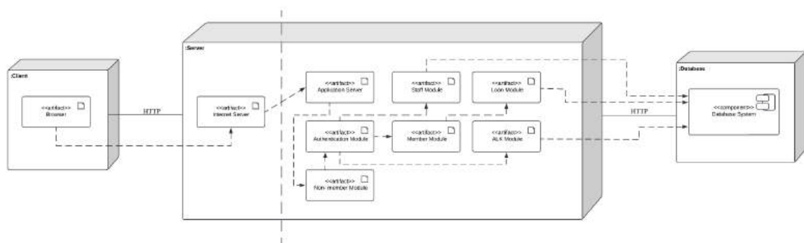
Figure 74: Deployment diagram for Koperasi KADA system
