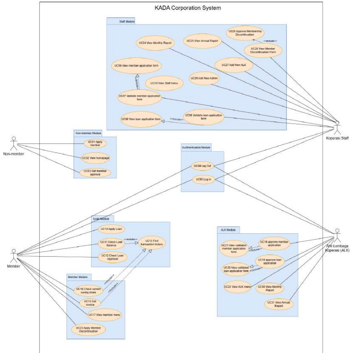
Figure 1: Use Case Diagram for Koperasi KADA System
