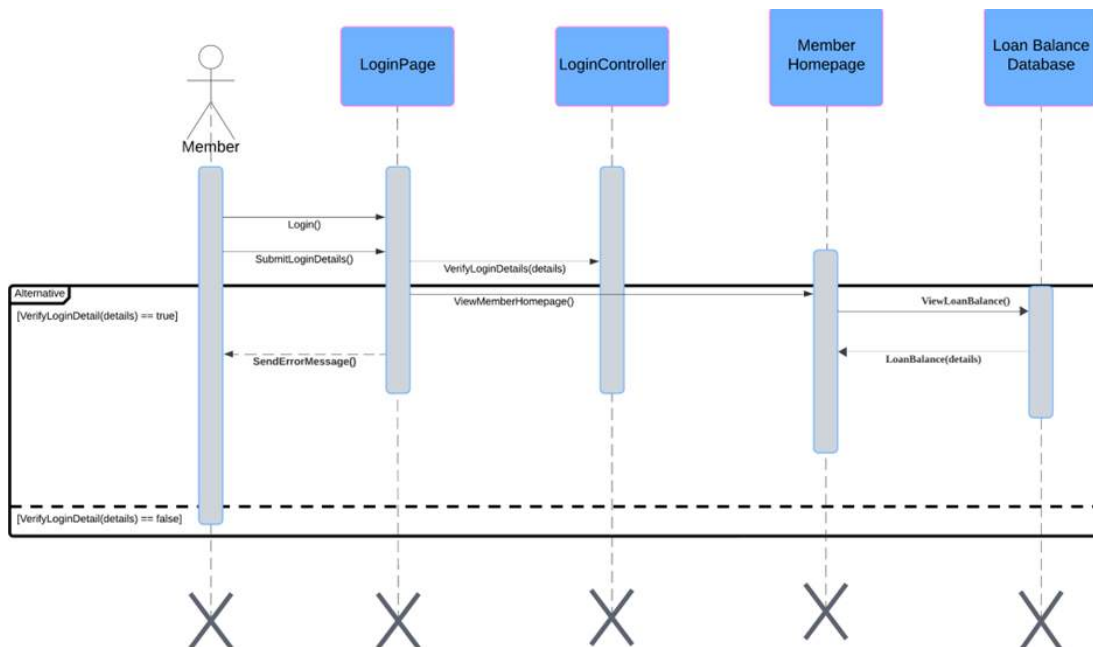
Figure 145: TC006_04: Test <Check Loan Balance (SD005)>
