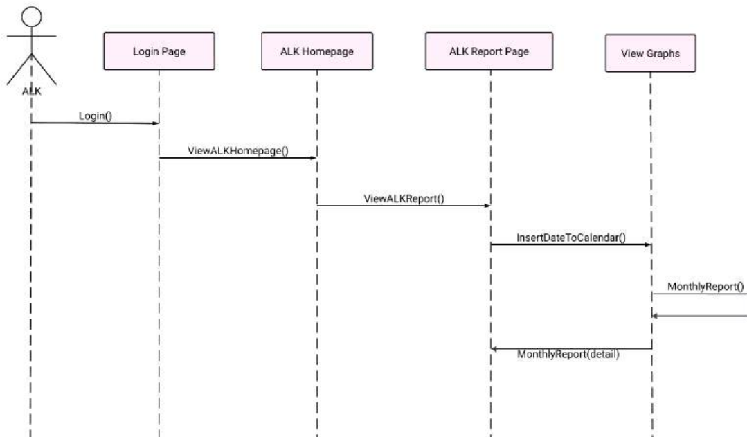
Figure 41: SD021 Sequence diagram for ALK view monthly report
