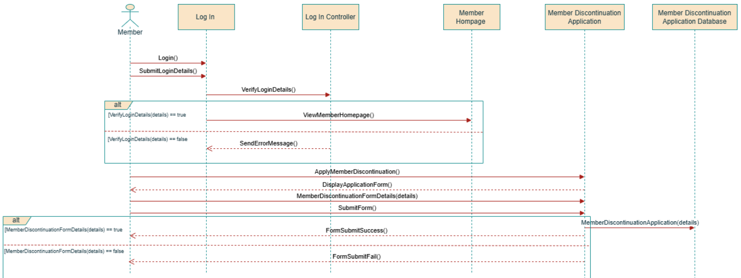
Figure 10: SD006 sequence diagram for apply membership termination
