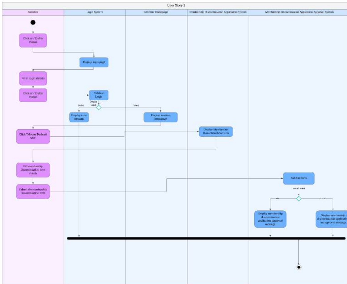
Figure 16: Activity diagram for member apply membership discontinuation
