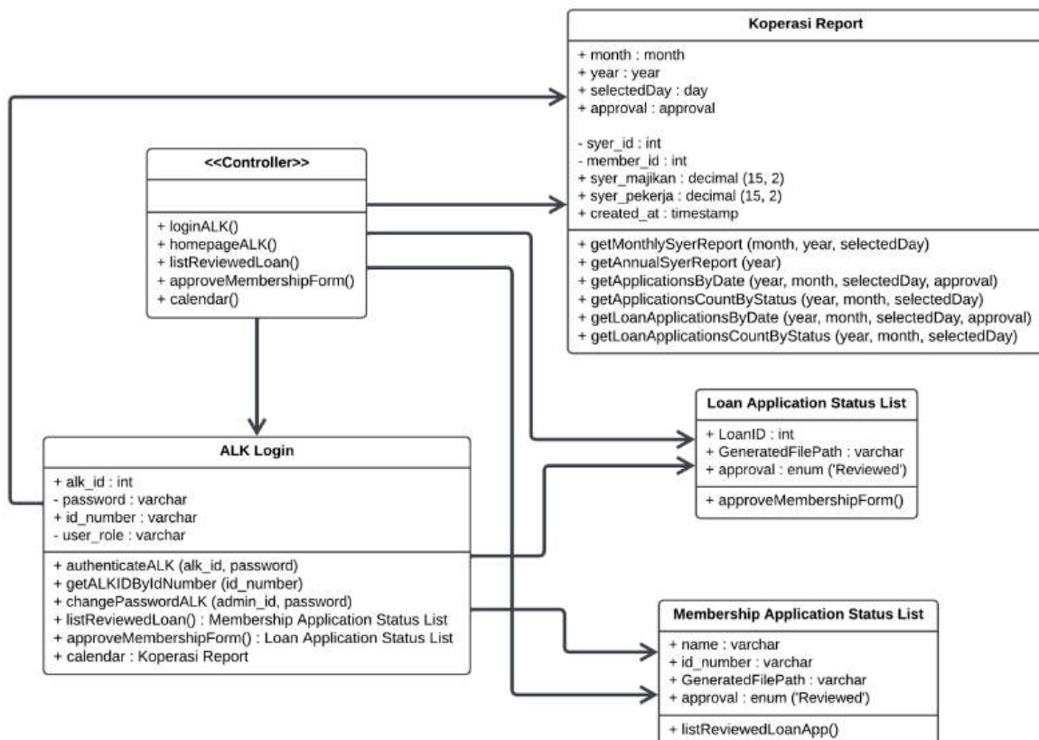
Figure 65: Class diagram for ALK module
