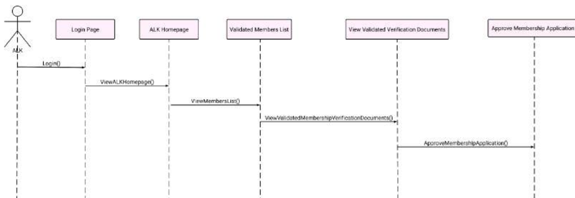
Figure 39: SD019 Sequence diagram for ALK approve membership applications
