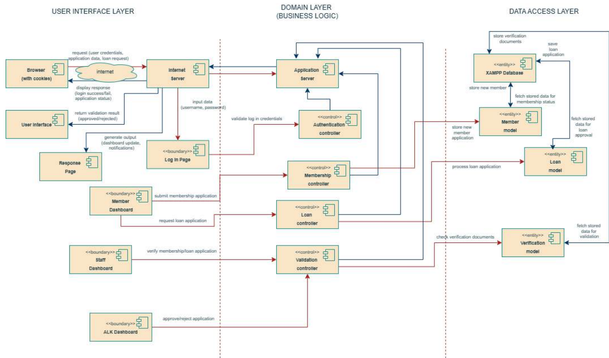
Figure 54: Component diagram of Koperasi KADA membership and loan application system
