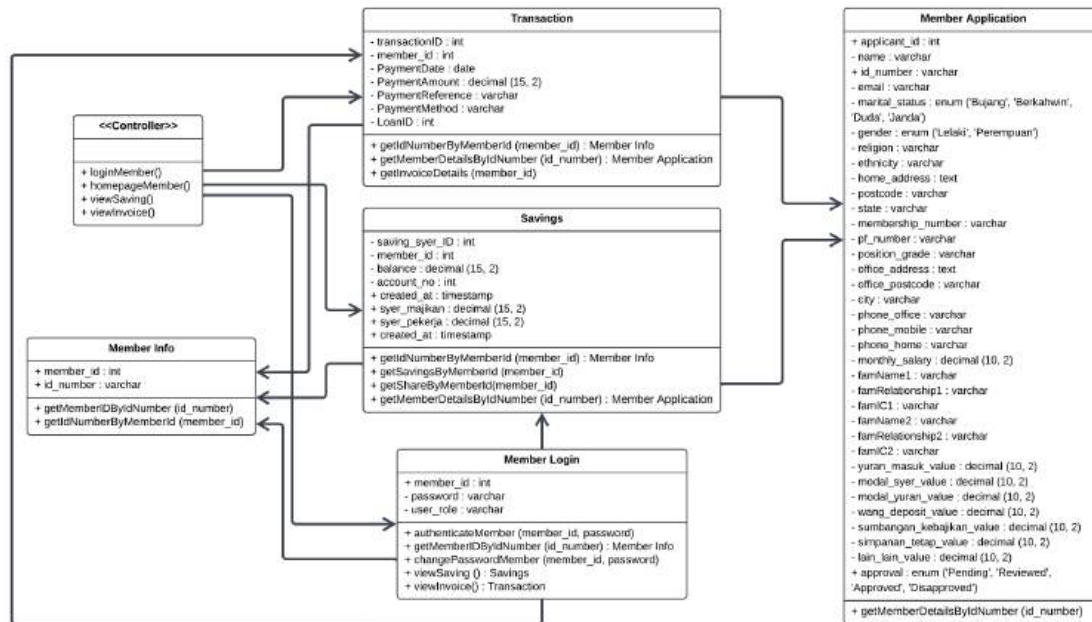
Figure 62: Class diagram for Member module
