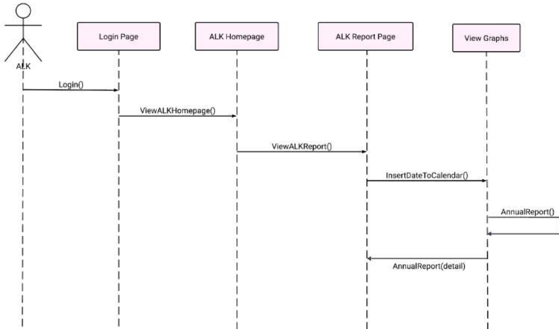
Figure 136: TC003_07: Test <View Annual Report (SD022)>
