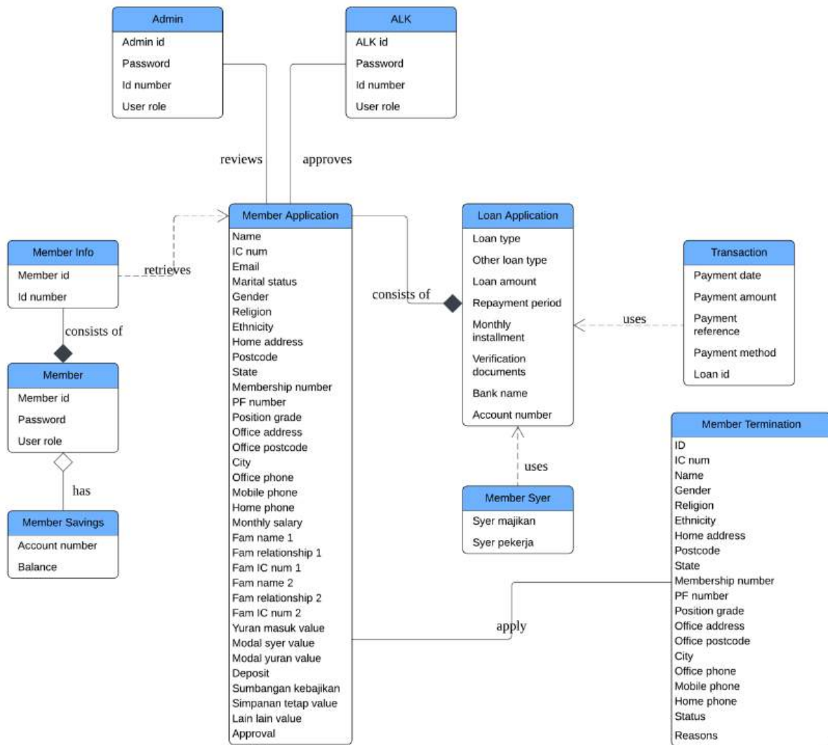
Figure 2: Domain Model for Koperasi KADA system
