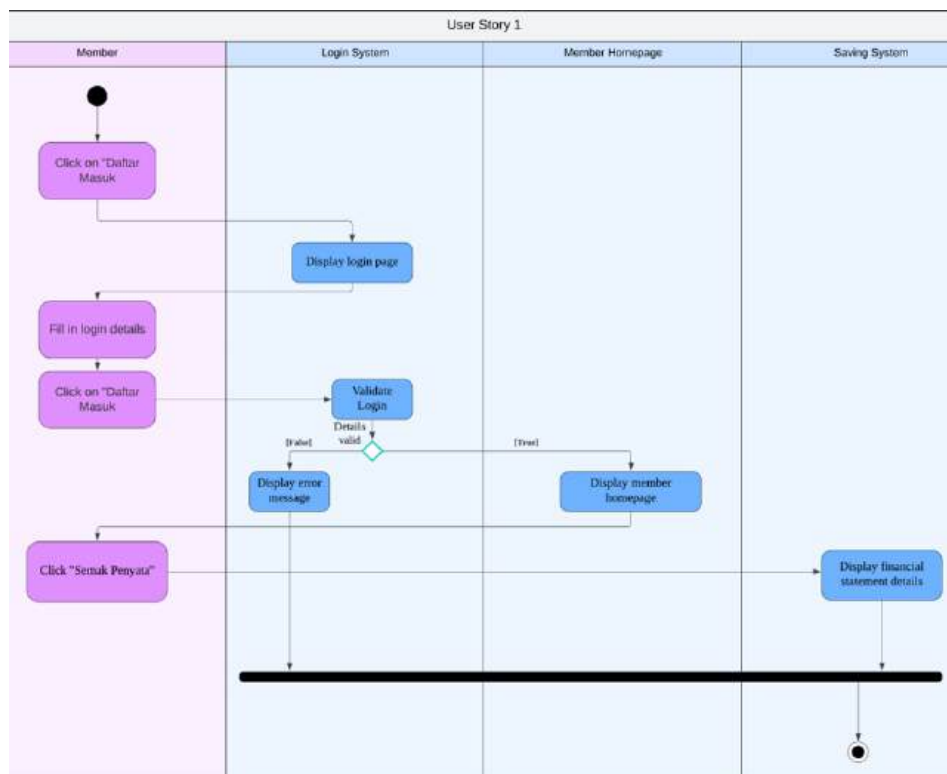
Figure 15: Activity diagram for member find transaction history
