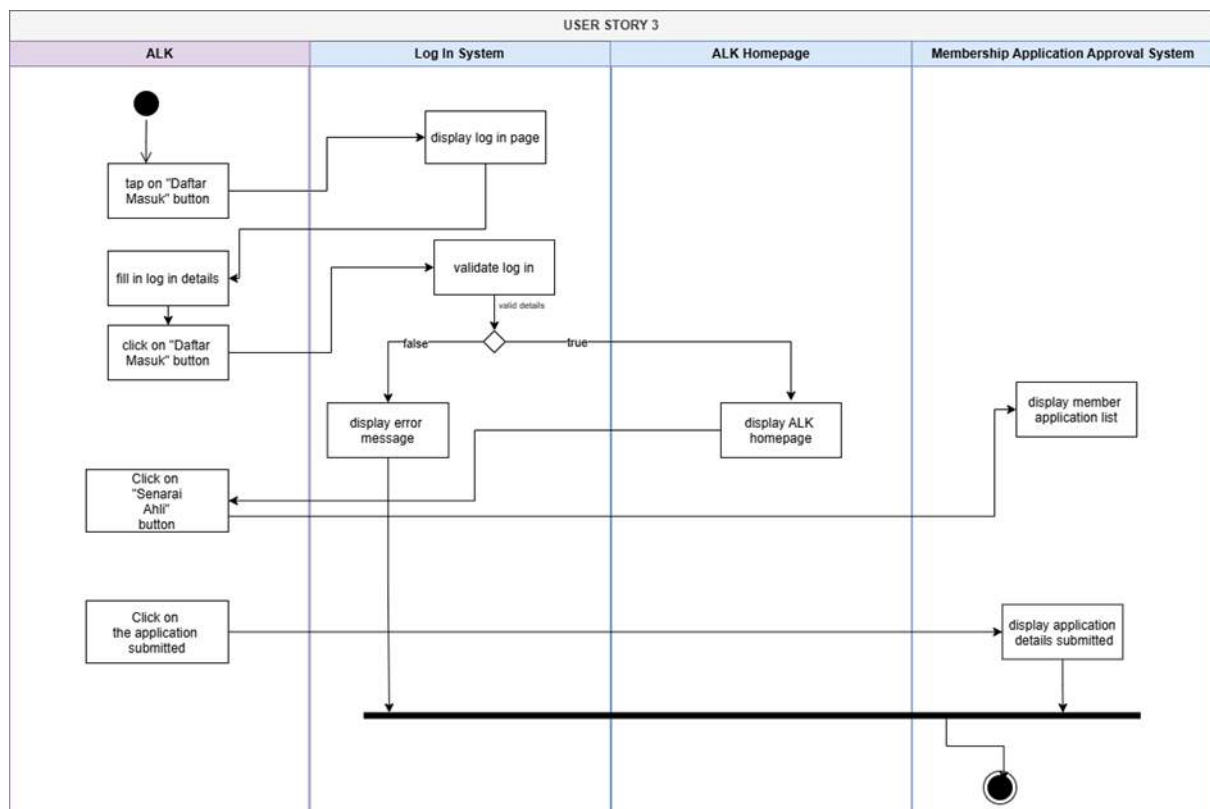
Figure 43: Activity Diagram for ALK view validated member application
