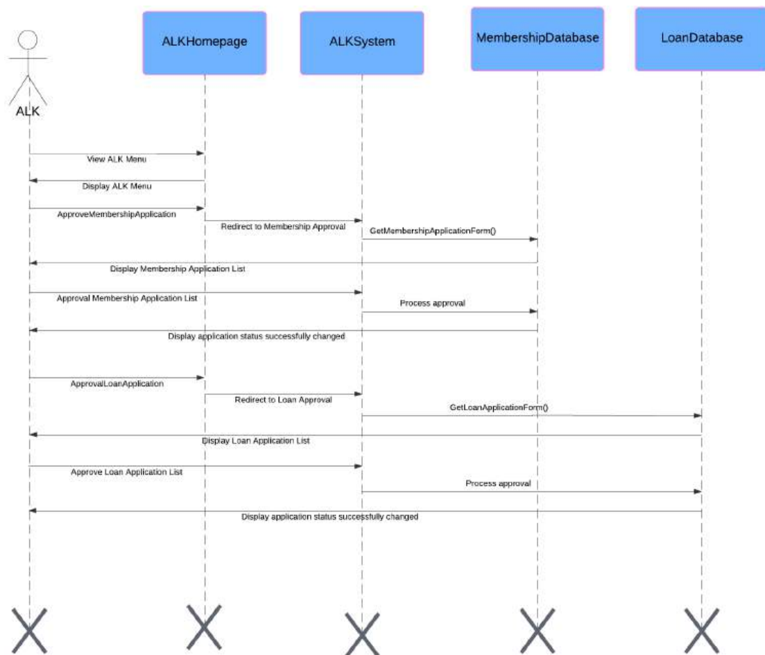
Figure 73: SD029 sequence diagram for ALK module
