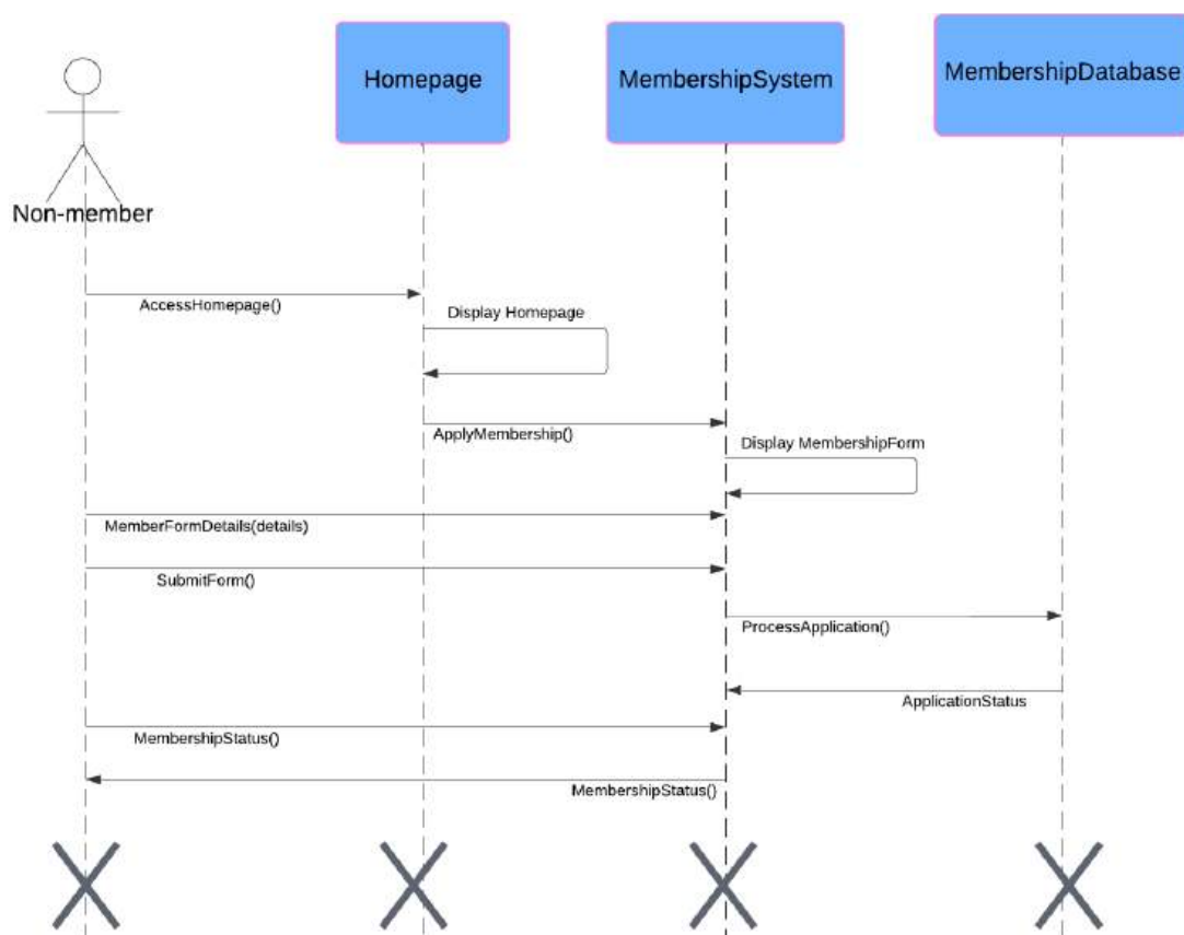
Figure 69: SD025 sequence diagram for Non-Member module
