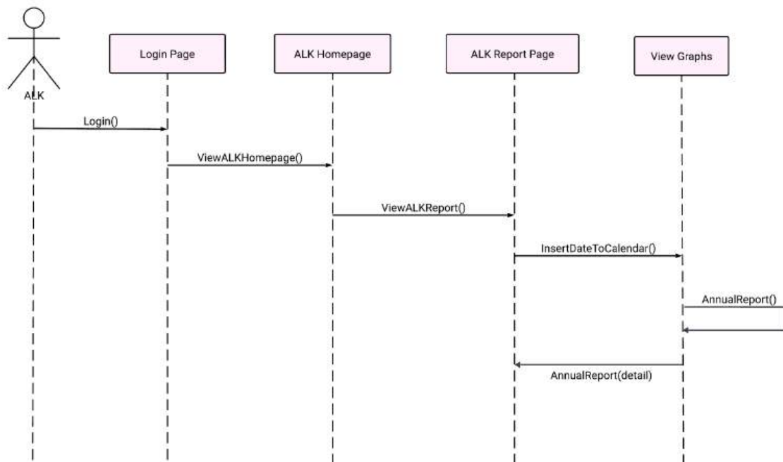
Figure 42: SD022 Sequence diagram for ALK view annual report
