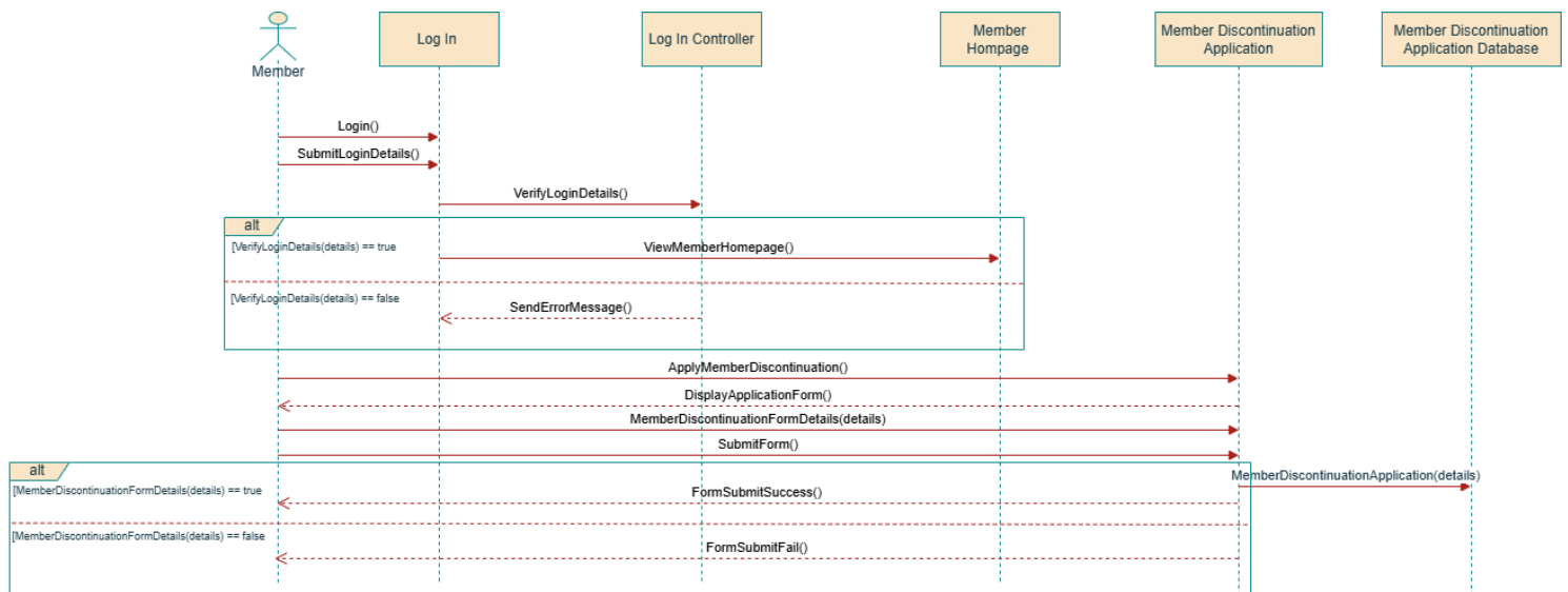
Figure 118: TC001_03: Test <Apply Membership Termination (SD006)>
