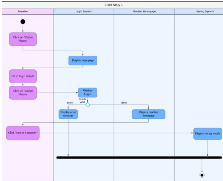
Figure 14: Activity diagram for member check current saving
